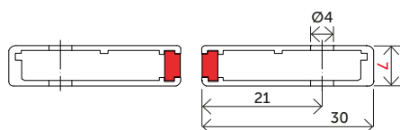
Mechanical profile
