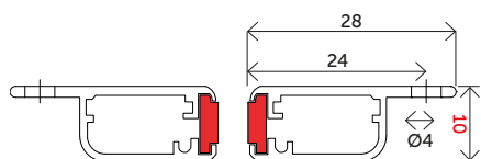
Mechanical profile
